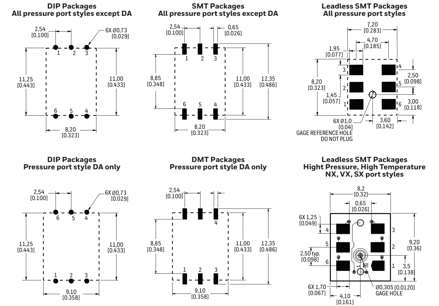
Figure 13. Recommended PCB Layout and Part Marking Details
